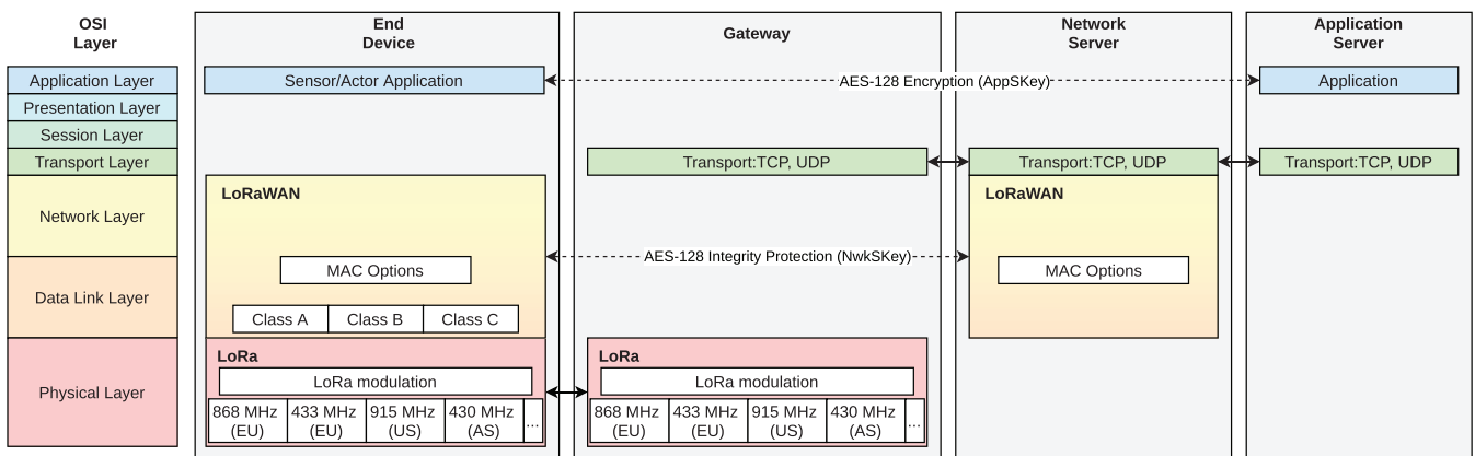
FIGURE 2 Simplified LoRaWAN technology stack in the OSI model (own illustration)
